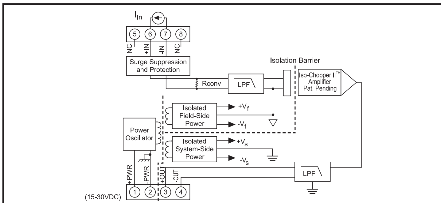
Figure 1: DSCA32 Block Diagram
